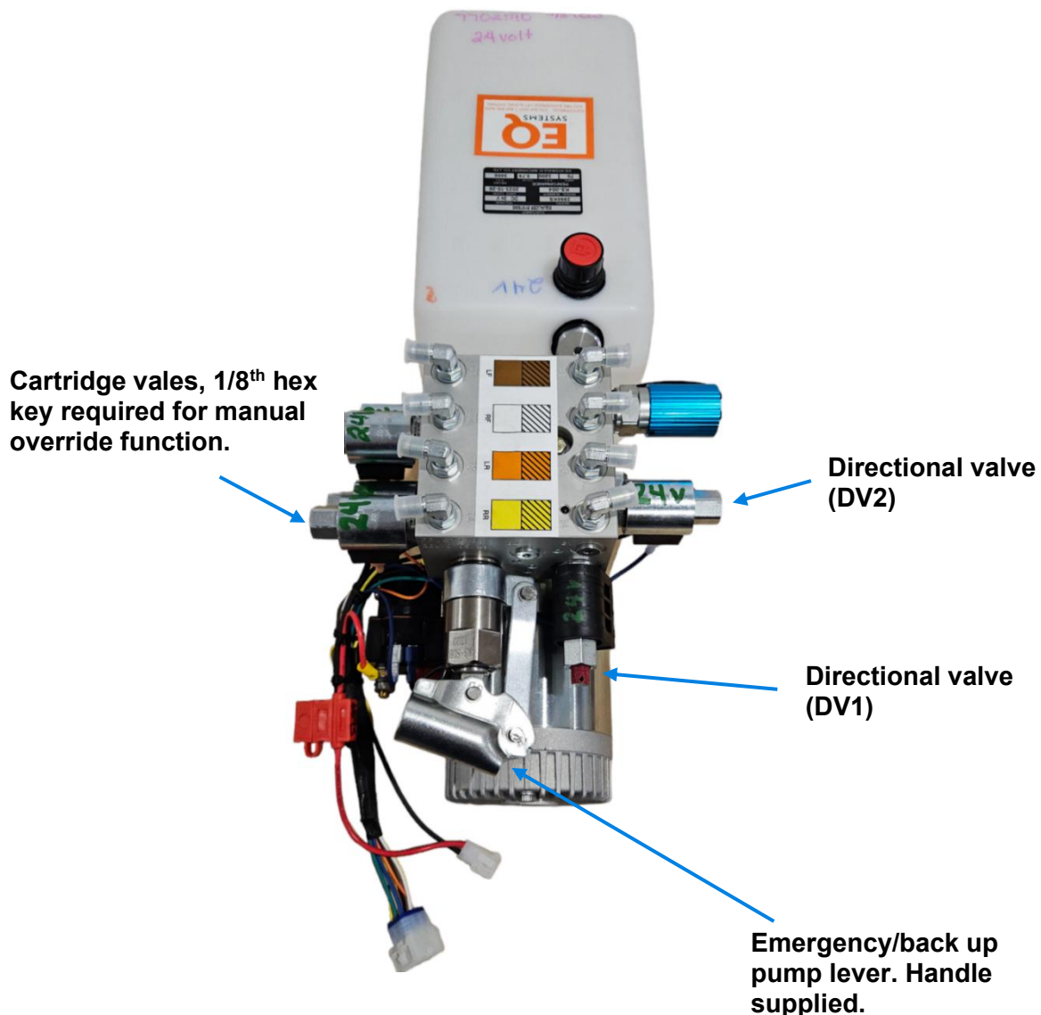
Figure 2. 7702MO-T Pump
